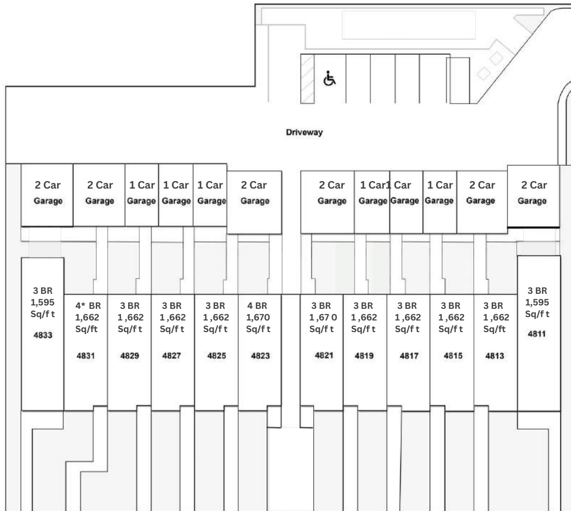
SITE PLAN
